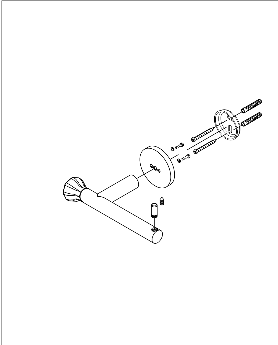
explosion diagram
