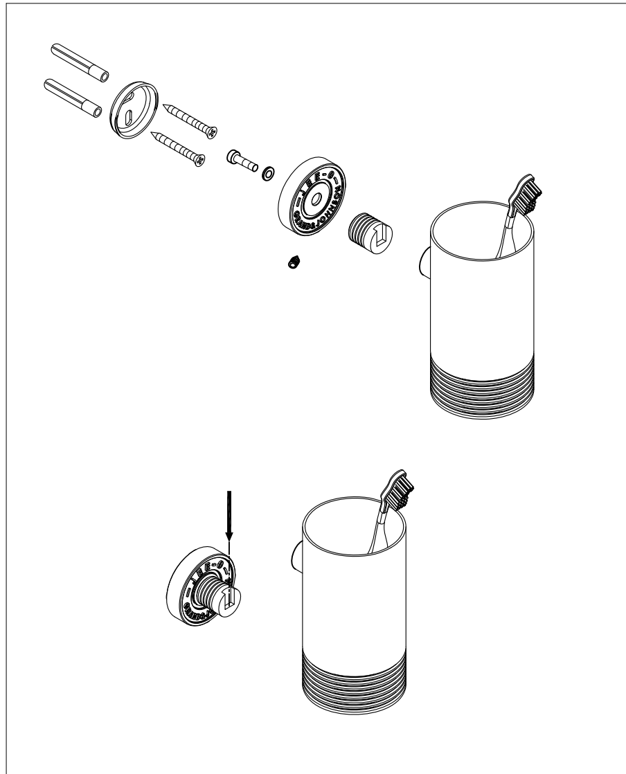
explosion diagram
